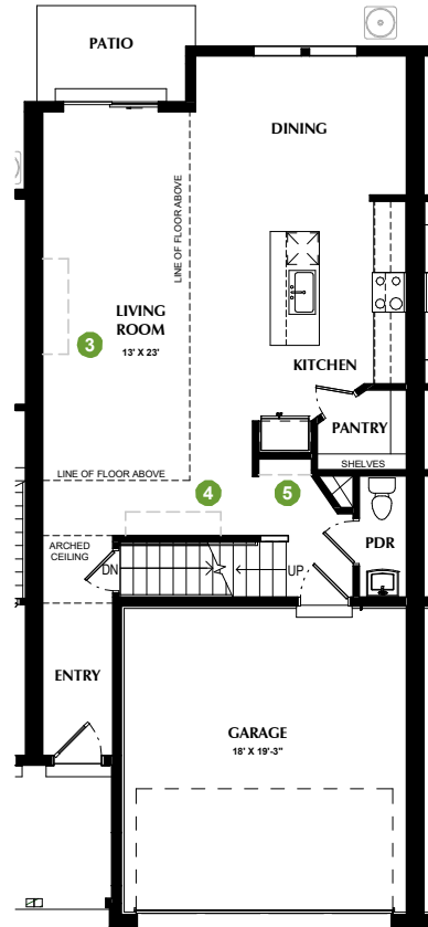
LEVEL 1 9' CEILINGS
