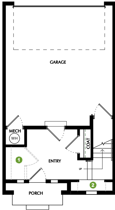
FIRST FLOOR 9' CEILINGS
