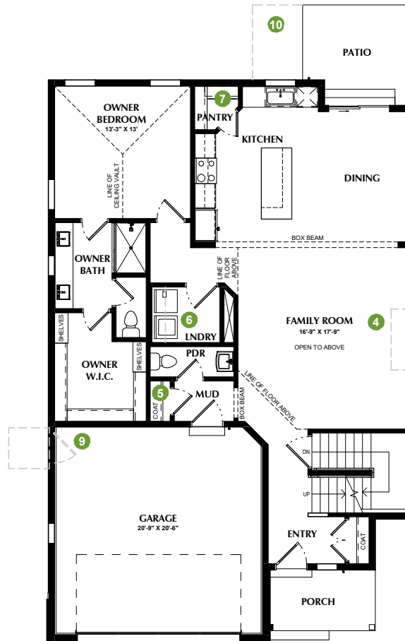
LEVEL 1 9' CEILINGS
