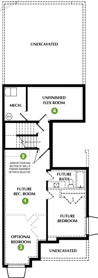
UNFINISHED BASEMENT
