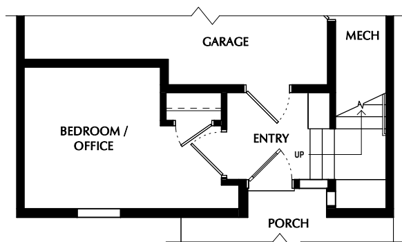
1 OPTION: FLEX ROOM (+121 SF) 9' CEILINGS
