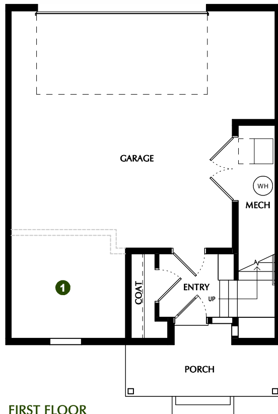
FIRST FLOOR 9' CEILINGS
