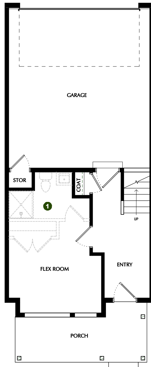
FIRST FLOOR 9' CEILINGS
