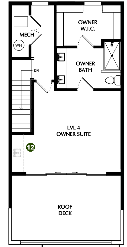
13 OPTION - LEVEL 4 OWNER SUITE 9' CEILINGS
